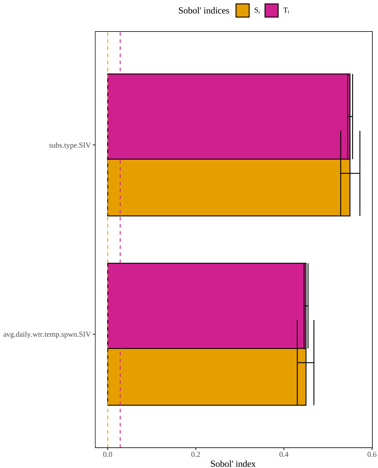
Figure 4. Results of a sensitivity analysis for the blueherringSAEL model based on an arithmetic mean structure. Dashed lines represent baseline numerical approximation error for S_i and T_i ( i.e. , dummy variables).
